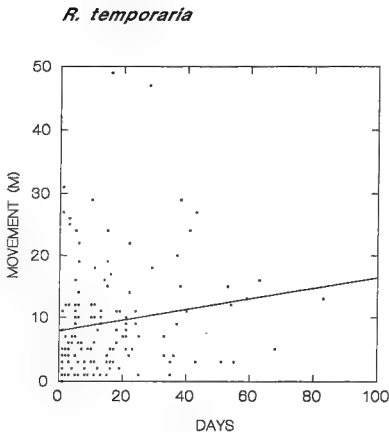
Fig. 2. - Relation of time between two captures and distance between the two sites. The correlation is significant for both species ( R. arvalis : r = 0.23 , d.f. = 101, P = 0.010 ; R. temporaria : r = 0.16 , d.f. = 137, P = 0.024 ). If the degree of freedom-values are reduced to the number of different frogs involved, the values are still significant ( R. arvalis : d.f. = 78, P < 0.025 , R. temporaria : d.f. = 95, P < 0.05 ). All P-values are based on one-tailed tests.
